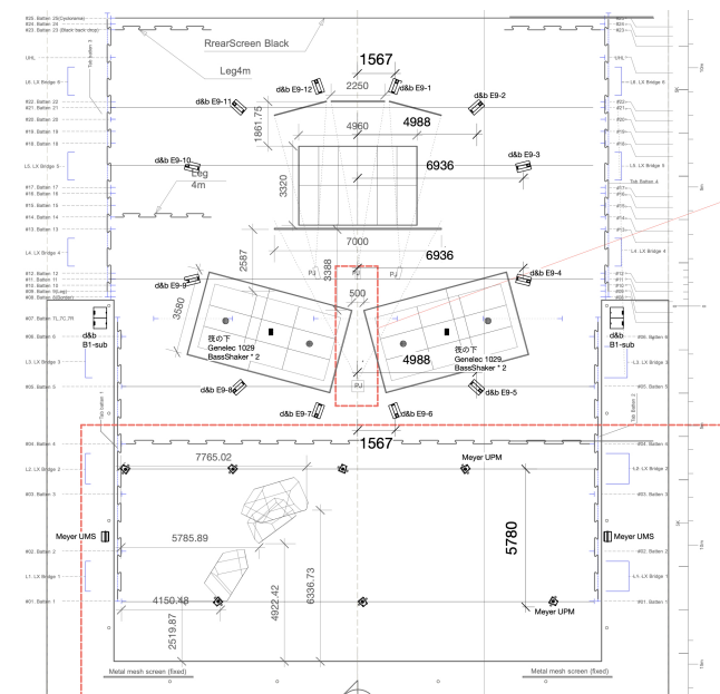
Figure 9: Speaker layout for both works (upper part: Another Capital Beneath the Waves , lower part: Crystal Seeding ). ©Tak-Cheung Hui
